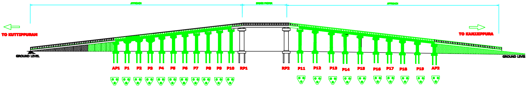
PILE FOUNDATION
